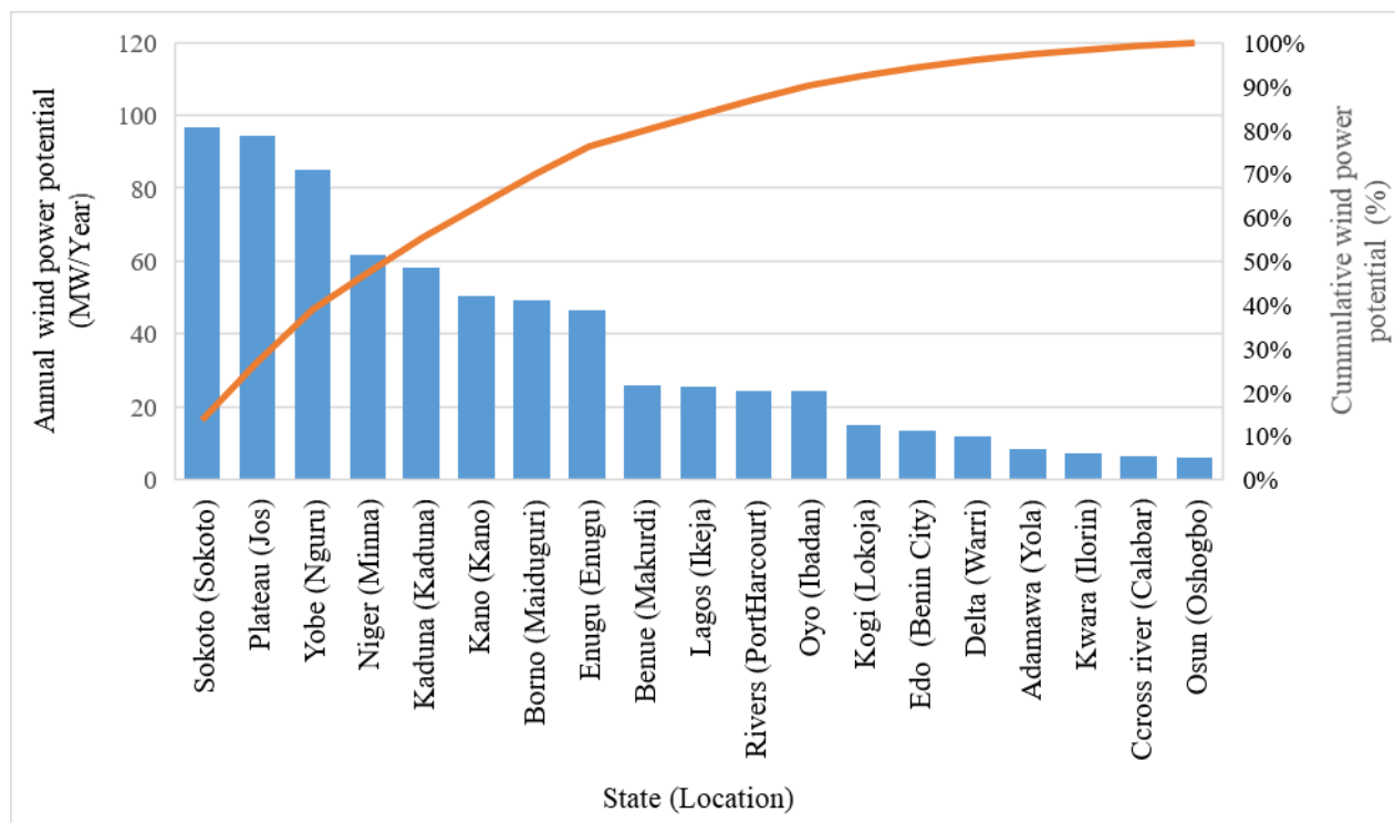
Fig. 2. Pareto plot for the distribution of Wind power potential in Nigeria
