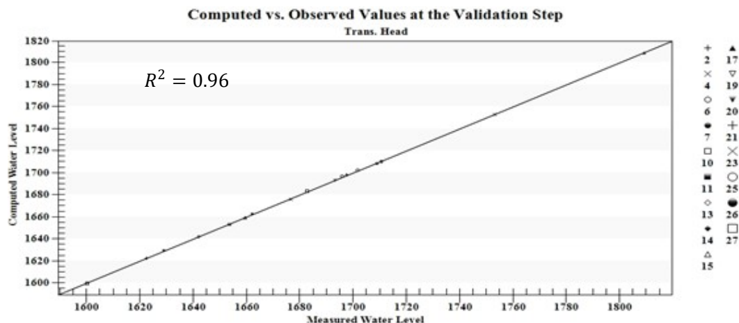
Fig. 9. Comparison plot of measured and computed water levels during the validation period
