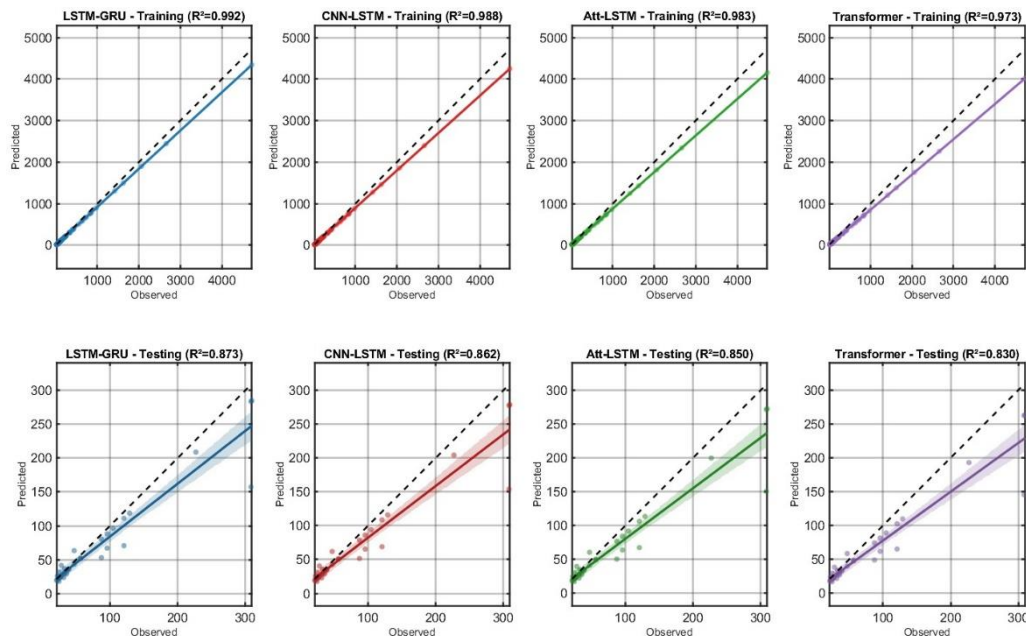
Fig. 2. Scatter plots of observed versus predicted inflow values for training and testing phases across four hybrid machine learning models.
