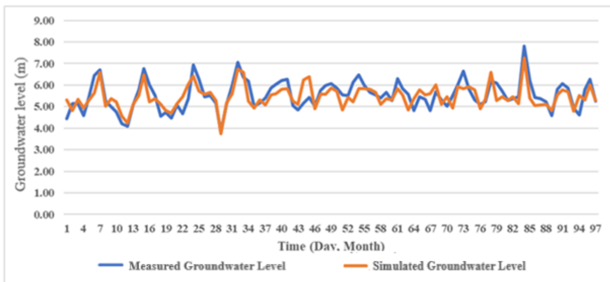
Fig. 6. Simulation of groundwater level (m) using Clayton's 2D copula
