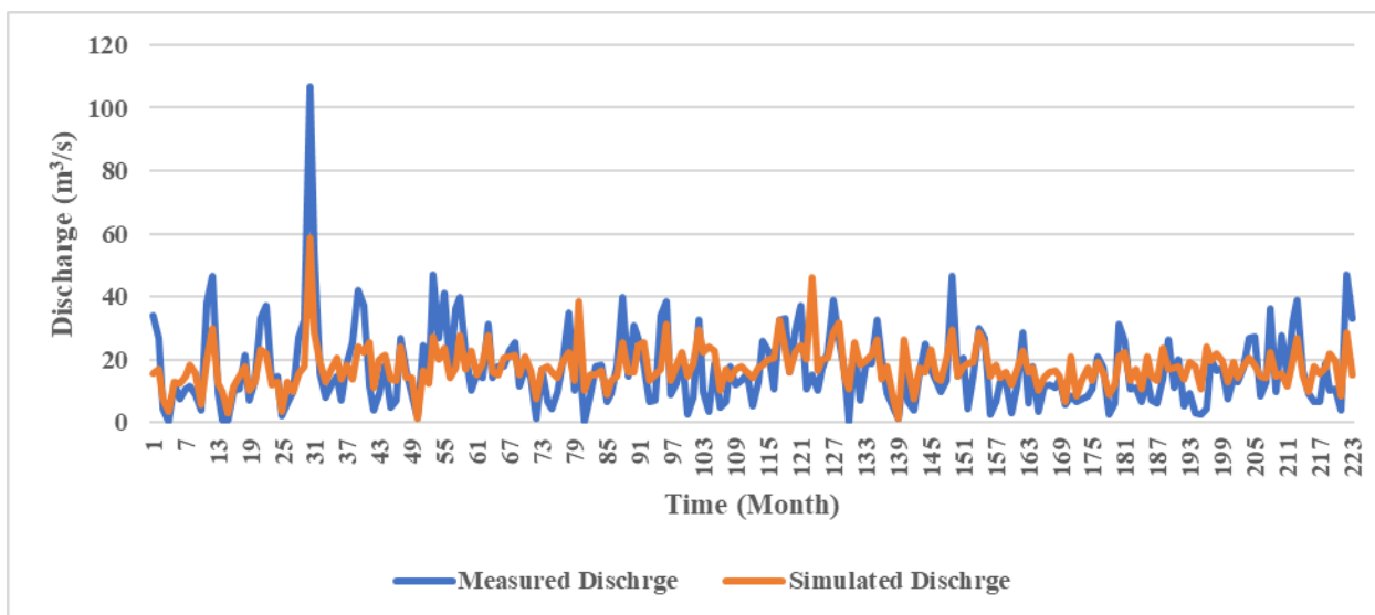
Fig. 5. Simulation of monthly river discharge ( m^3/s ) using Clayton's 2D copula
