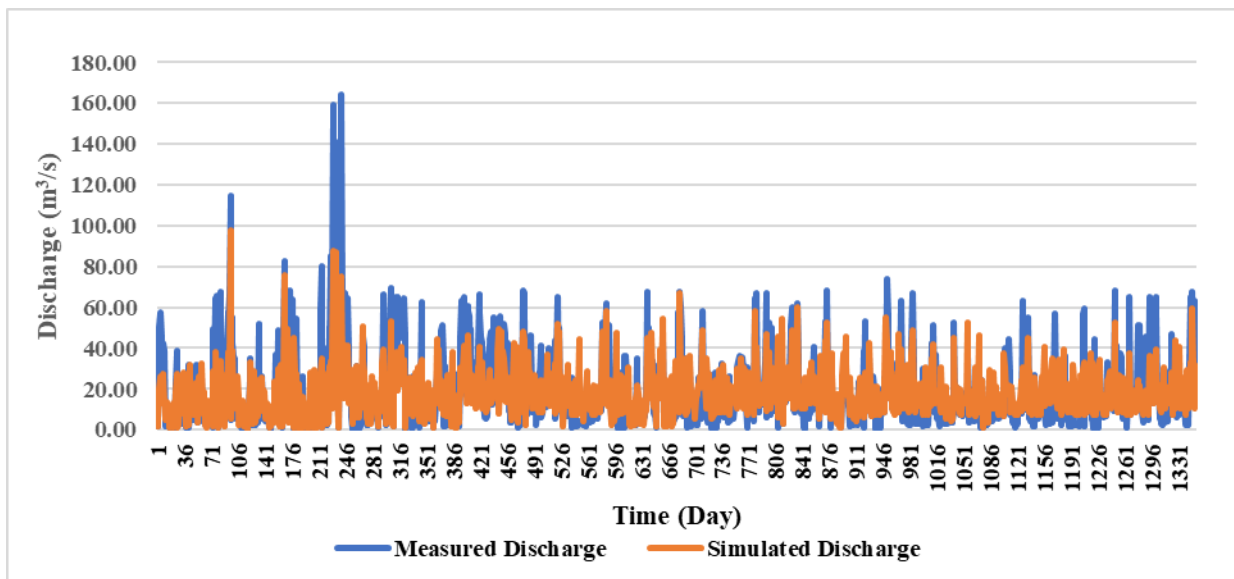
Fig. 4. Simulation of daily river discharge (m 3 /s) using Clayton's 2D copula
